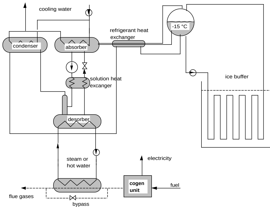
Figure 6 Diagram of the ARP in cobination with an ice buffer as installed in a dairy factory in Burgos (Spain)
