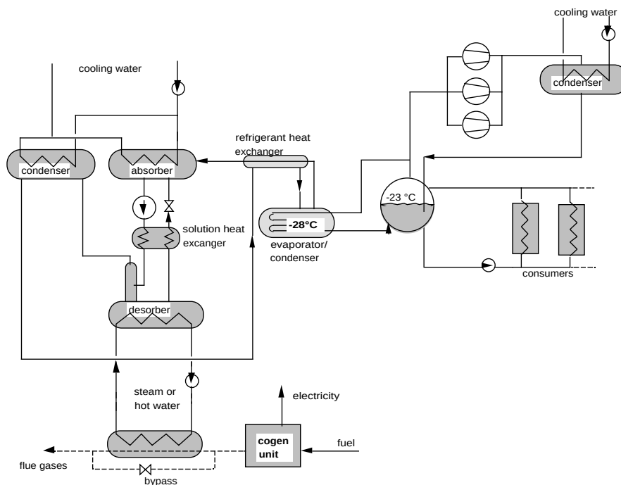
Figure 2 Diagram of the ARP installed in combination with a compression refrigeration plant in a margarine factory in Rotterdam (Netherlands).
